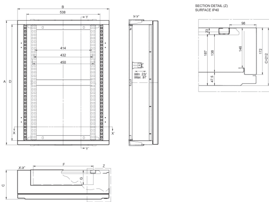
Standard drawing
